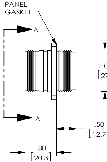
PANEL GASKET
