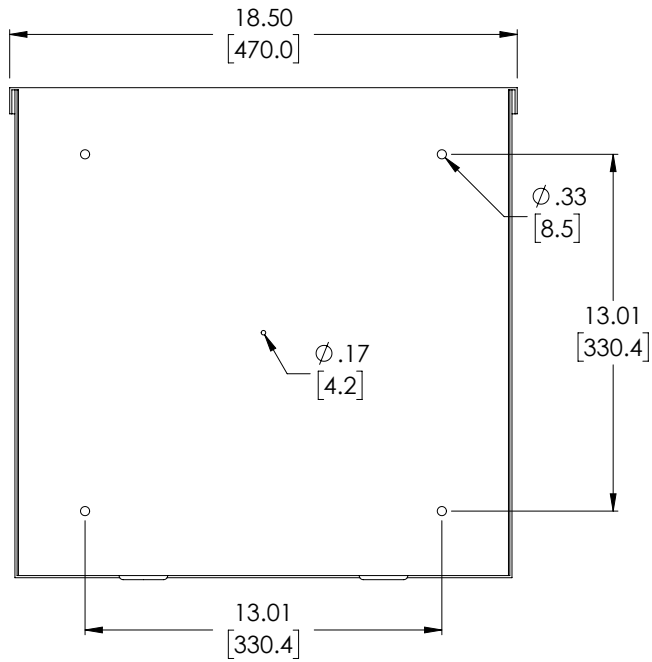
BOTTOM VIEW
