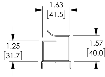
SECTION A-A SCALE 1 : 3.5
