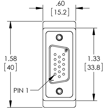
"P1" 15-PIN MALE HIGH DENSITY D-SUB CONNECTOR
