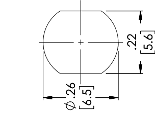
Recommended Mounting Hole
