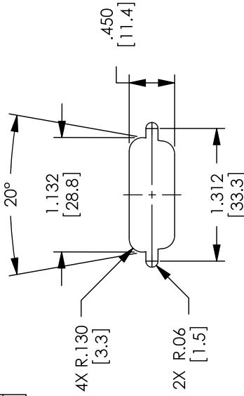
RECOMMENDED PANEL OPENING (MAX PANEL THICKNESS: 0.06")
