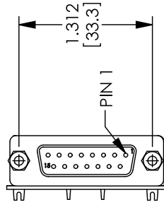
DB15 FEMALE D-SUB CONNECTOR
