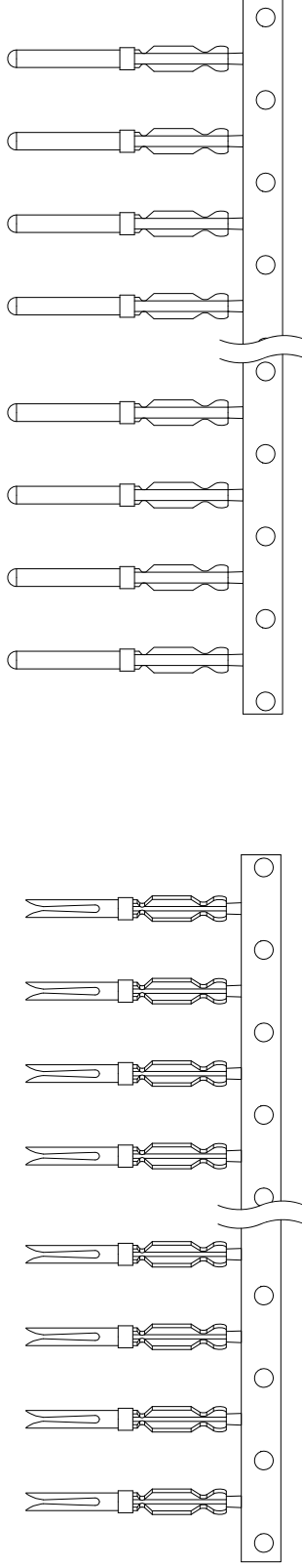
STANDARD FEMALE CONTACTS, 24-28 AWG
