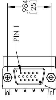
MALE 15 CONTACT HIGH DENSITY D-SUB CONNECTOR
