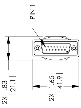
"P1" 2X, DB15 MALE CONNECTOR
