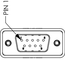
"P1" MALE 9-PIN D-SUB CONNECTOR
