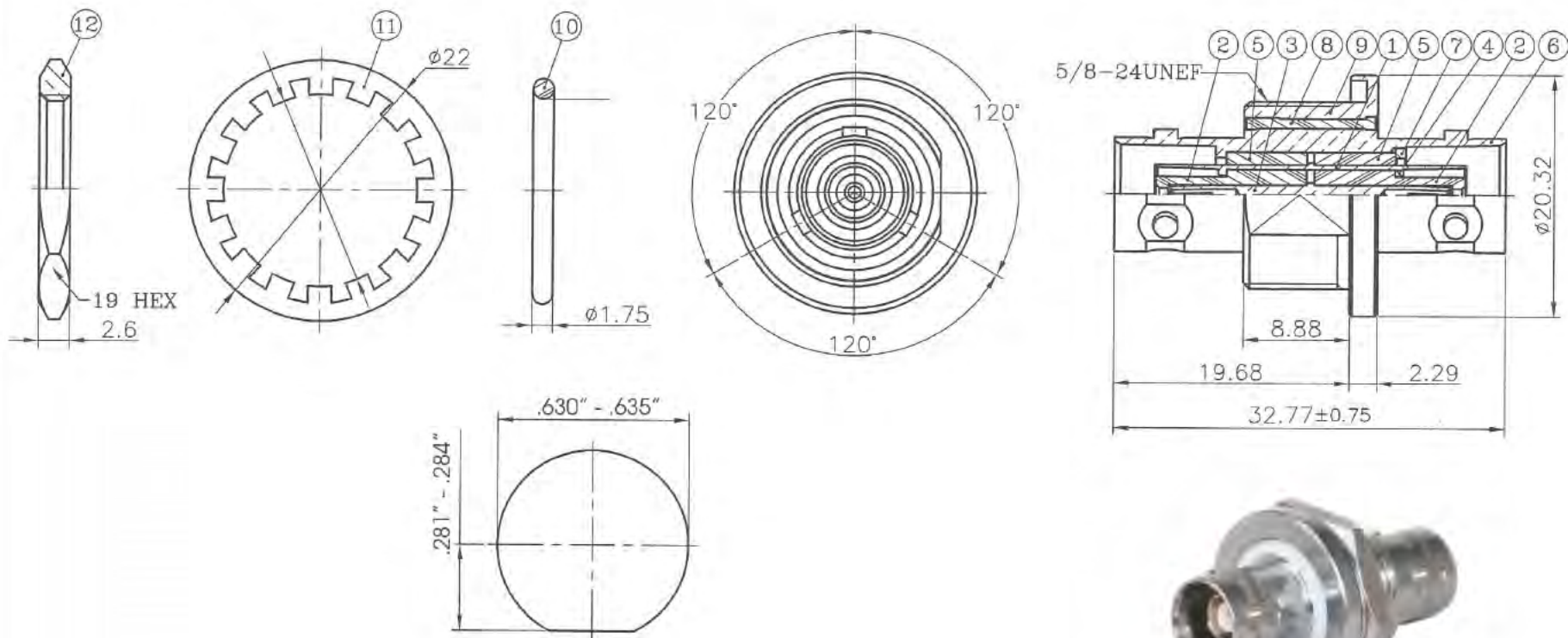
RECOMMENDED MOUNTING HOLE DIMENSIONS (inches)
