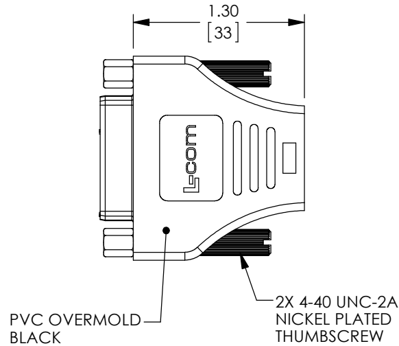
"J2" FEMALE HDMI CONNECTOR BLACK INSULATOR NICKEL PLATED SHELL
