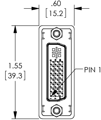
"J1" FEMALE DVI-I CONNECTOR (WHITE INSULATOR)
