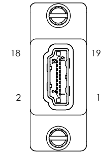
"J2" FEMALE HDMI CONNECTOR BLACK INSULATOR NICKEL PLATED SHELL
