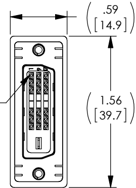
"P1" MALE DVI-D SINGLE LINK CONNECTOR
